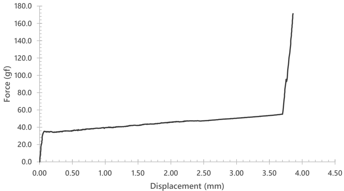
Cherry MX Lumina Red (Upstroke)
